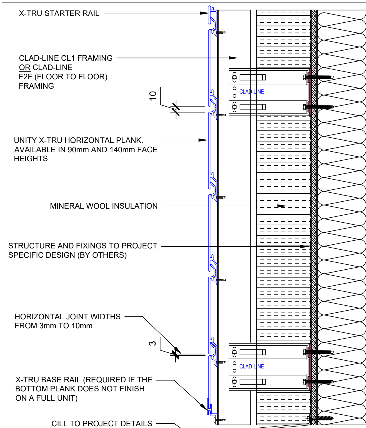
UNITY X-TRU TYPICAL HORIZONTAL JOINT DETAIL (HORIZONTAL PLANK)
